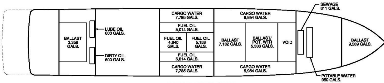
TANK ARRANGEMENT
