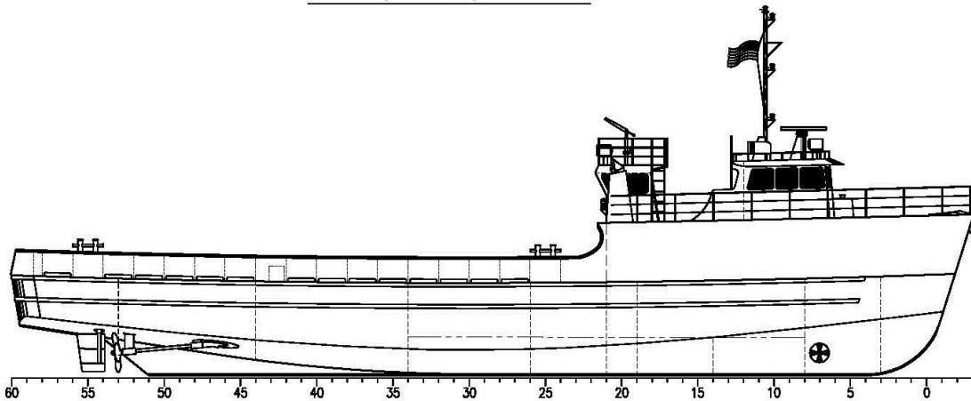
OUTBOARD PROFILE
