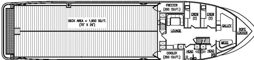
MAIN DECK ARRANGEMENT PLAN
