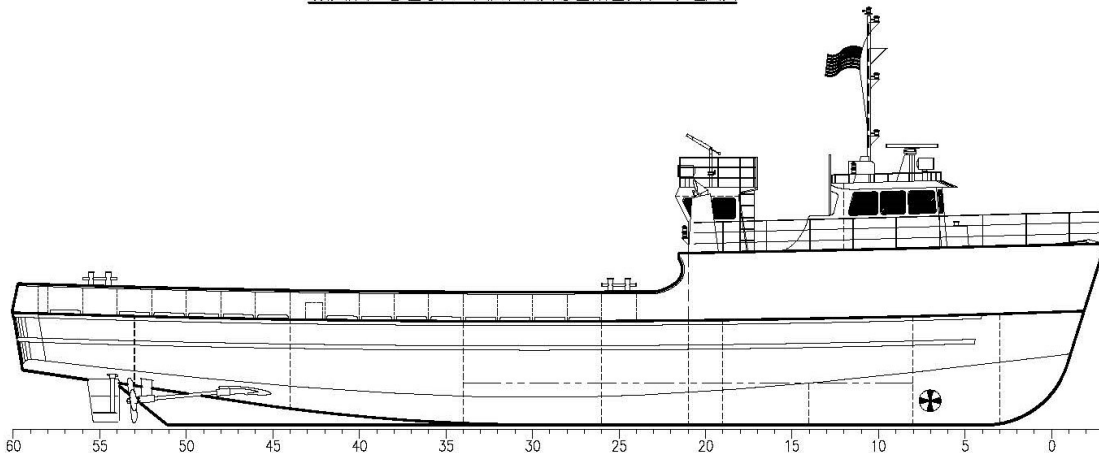
OUTBOARD PROFILE
