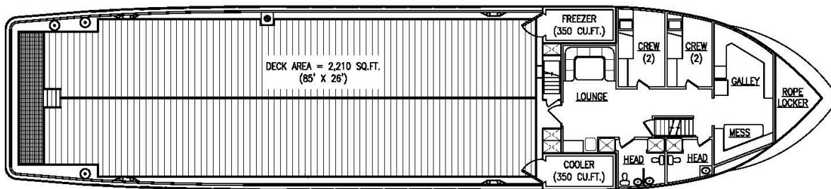
MAIN DECK ARRANGEMENT PLAN
