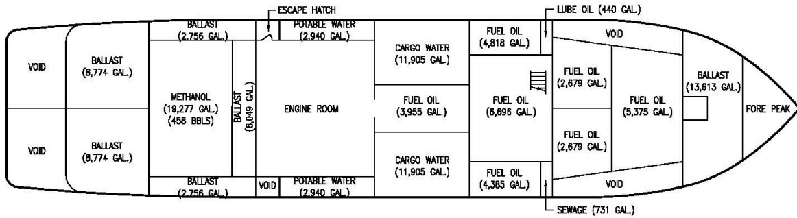
TANK ARRANGEMENT PLAN
